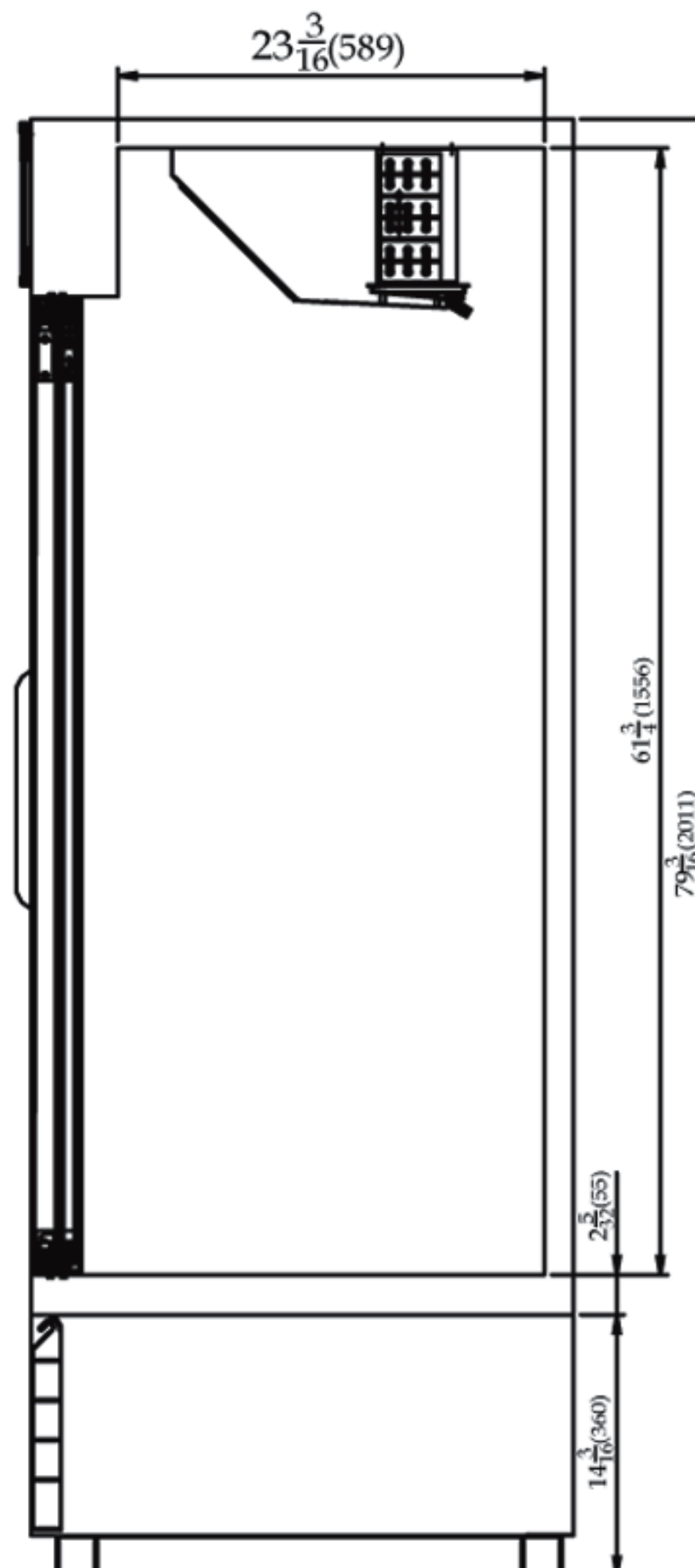
TGM-69R SIDE VIEW
