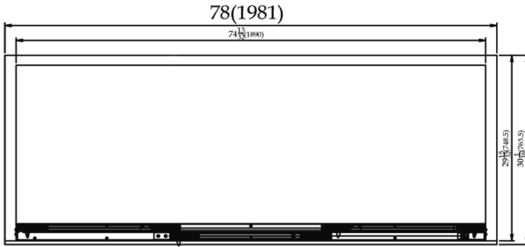
TGM-69R PLAN VIEW
