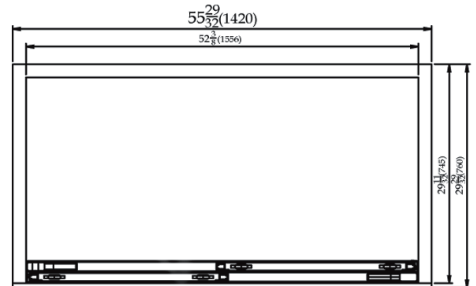
TGM-48R PLAN VIEW
