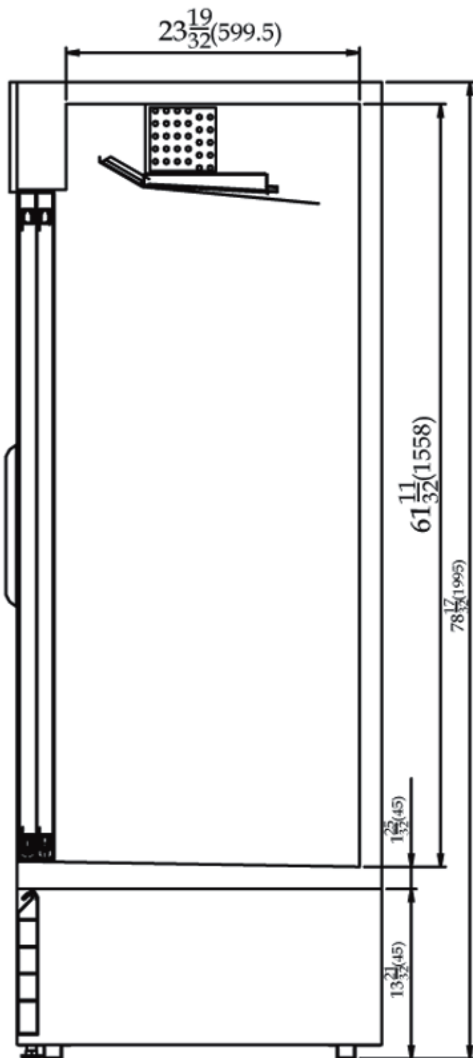
TGM-35R/48R SIDE VIEW
